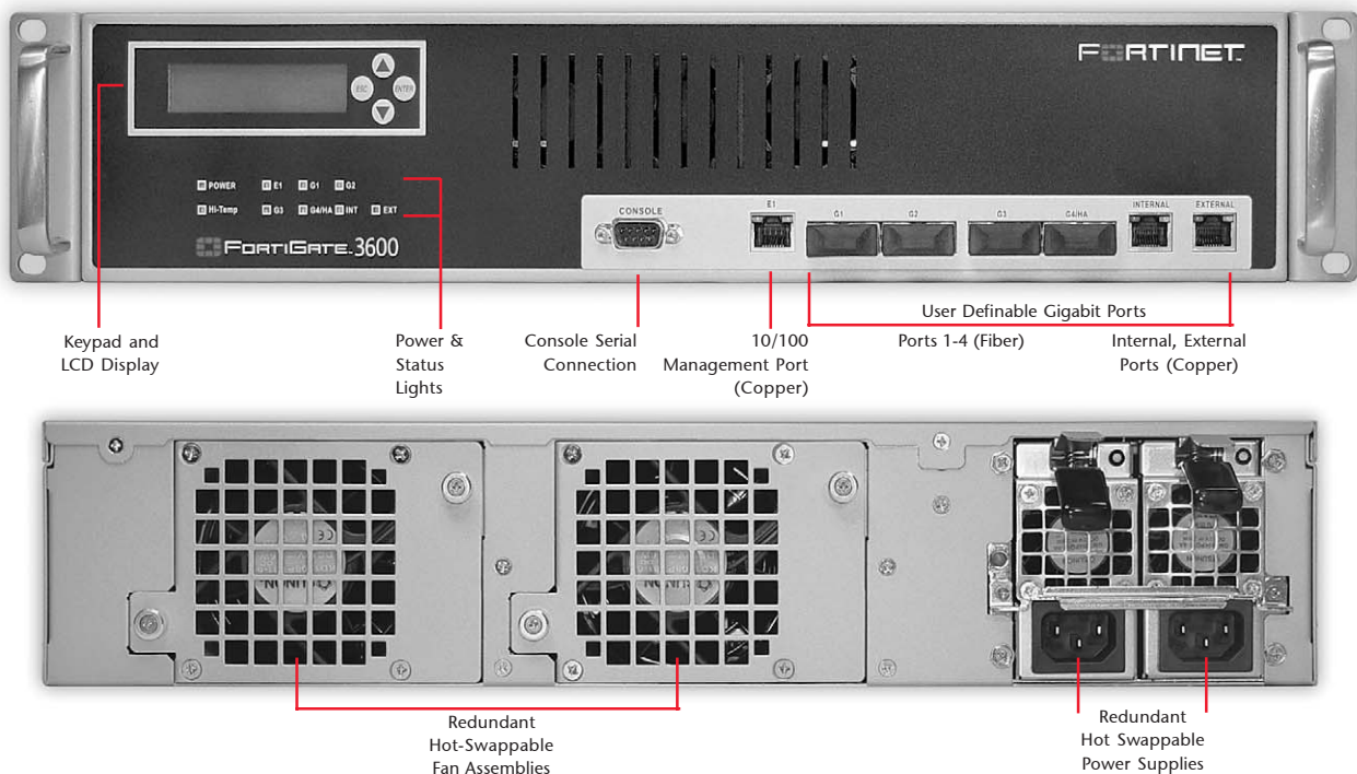
FortiGate-3600
